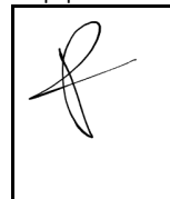
PENNEC Aaron
